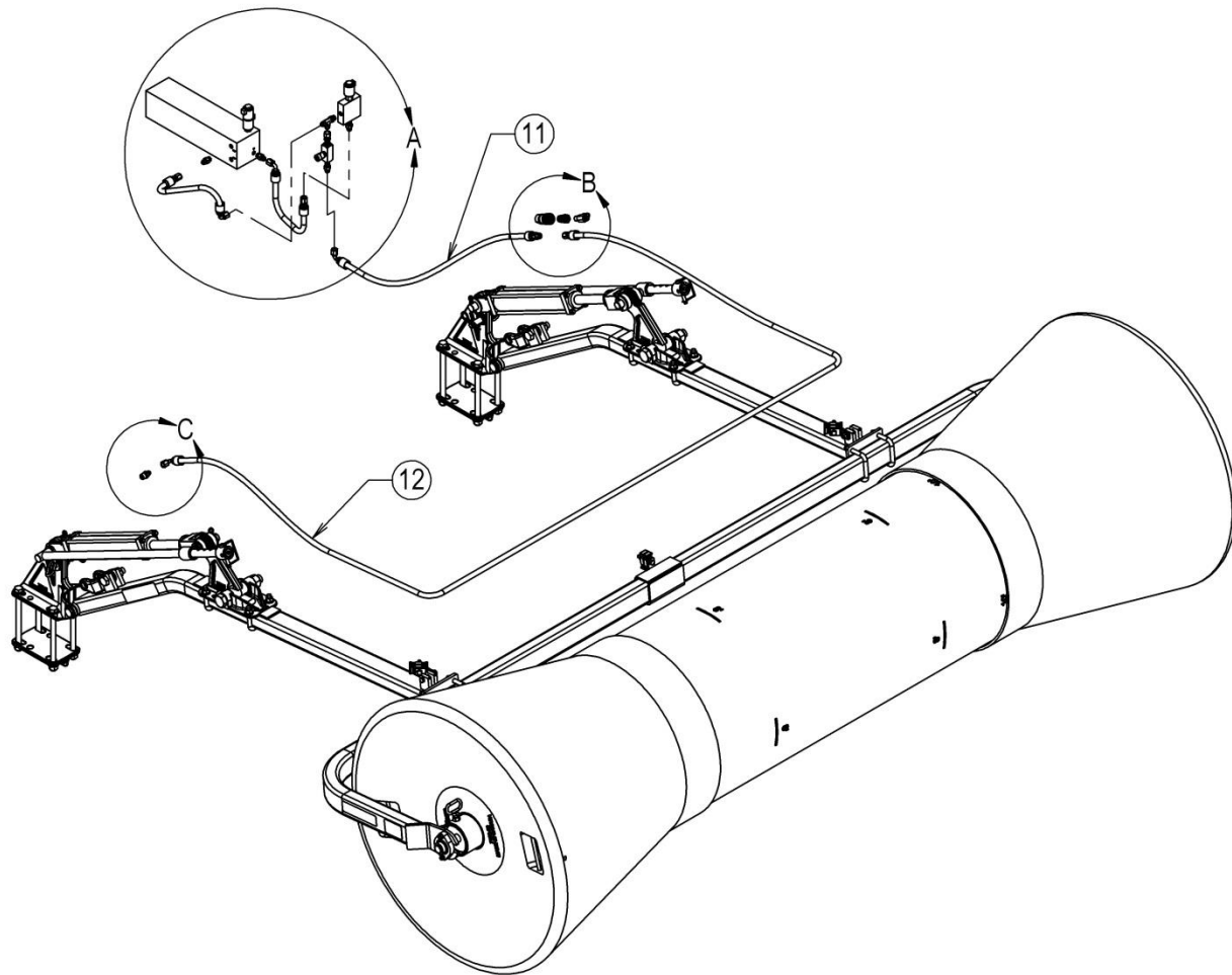
Figure 1 – Completed Assembly
